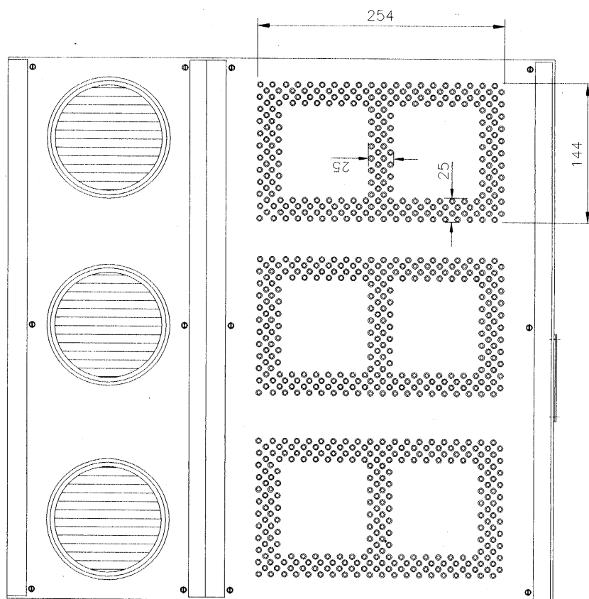
VISTA FRONTAL
