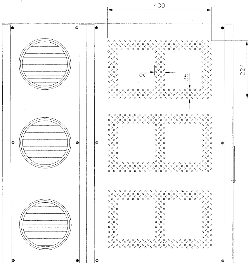
VISTA FRONTAL
